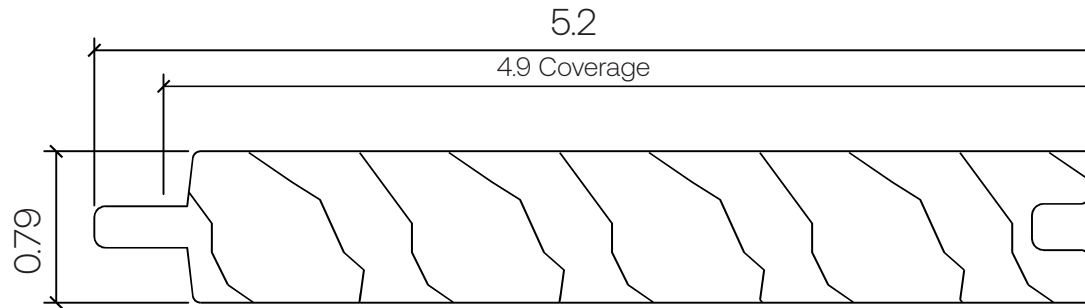
1x6 STANDARD CLADDING - C57 (JEM)
