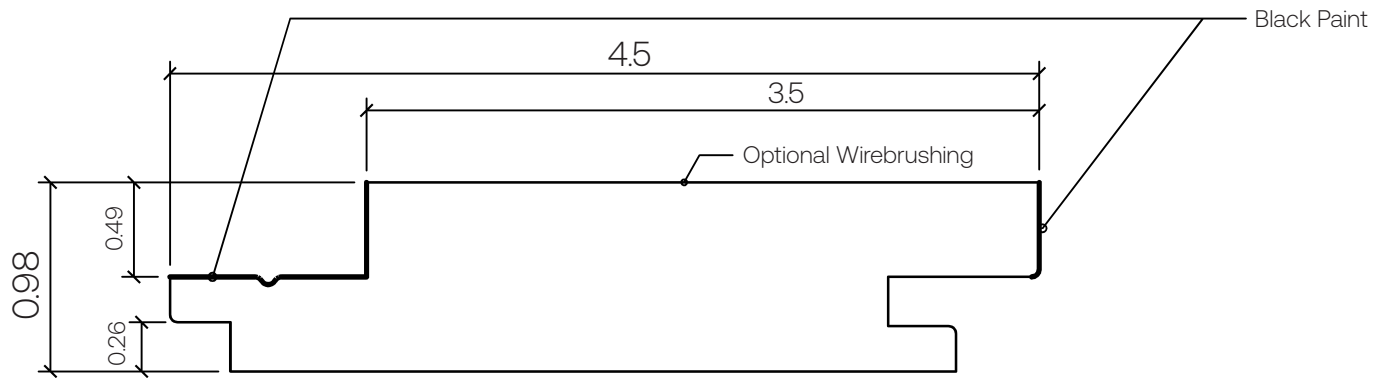
5/4 x 5 CLADDING - C34 STRIPES (SMOOTH OR BRUSHED)
