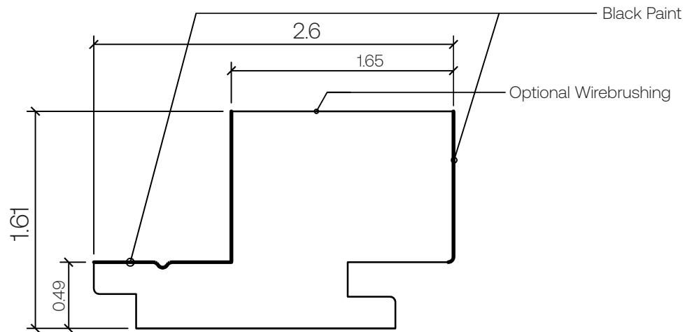
2x3 CLADDING - C34 STRIPES (SMOOTH OR BRUSHED)
