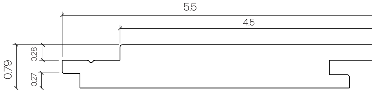
1 X 6 CLADDING - C34 Mix & Match (JEM)
