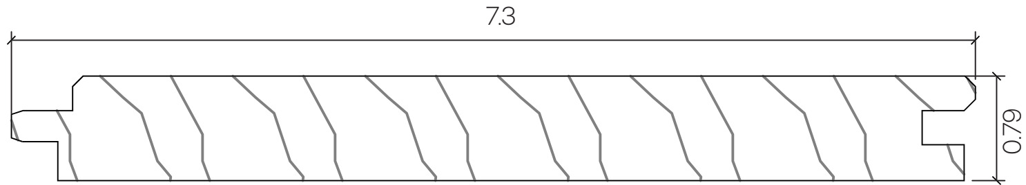
1X8 CLADDING - C15 GROOVED (JEM)
