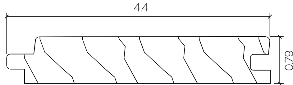
1x5 CLADDING - C20 (JEM)
